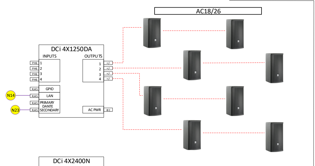
UNDER BALCONY DELAY SYSTEM
