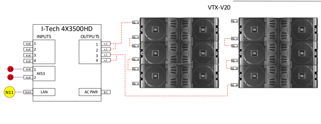
MAIN RIGHT ARRAY
