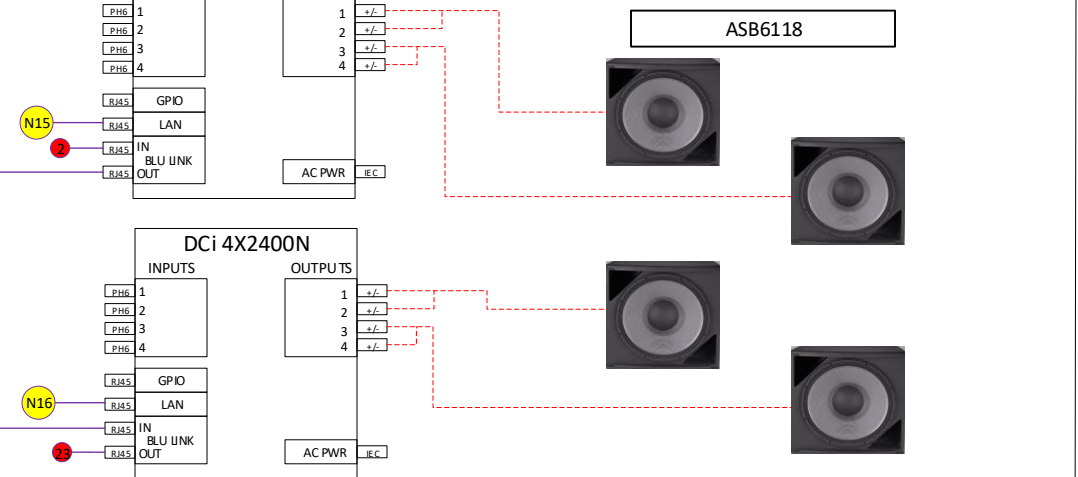
GROUND SUPPORT SUBWOOFERS
