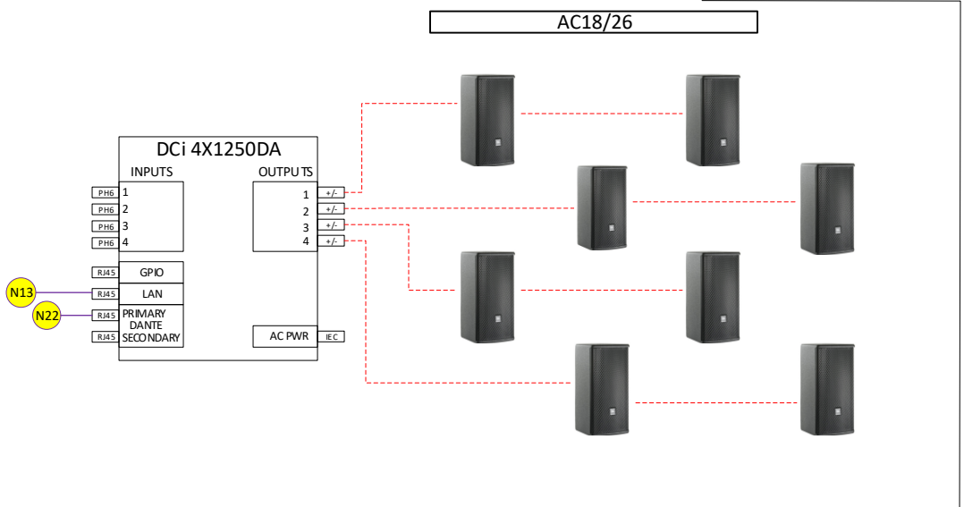
STAGE LIP PROXIMITY SYSTEM
